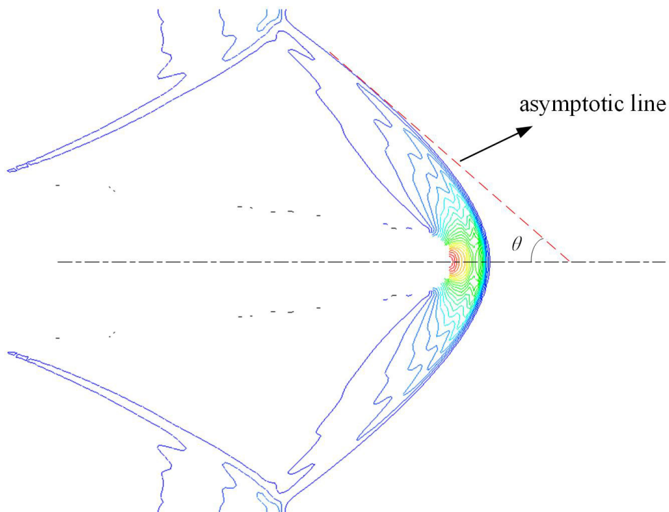
(b) Isobaric distribution in water
