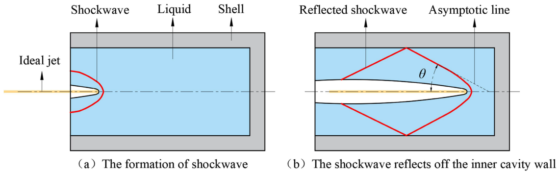
Figure 2 Propagation of shockwave in a liquid composite protective structure
