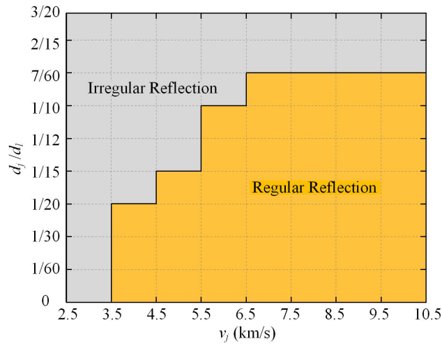
Figure 13 Distribution of shockwave reflection types
