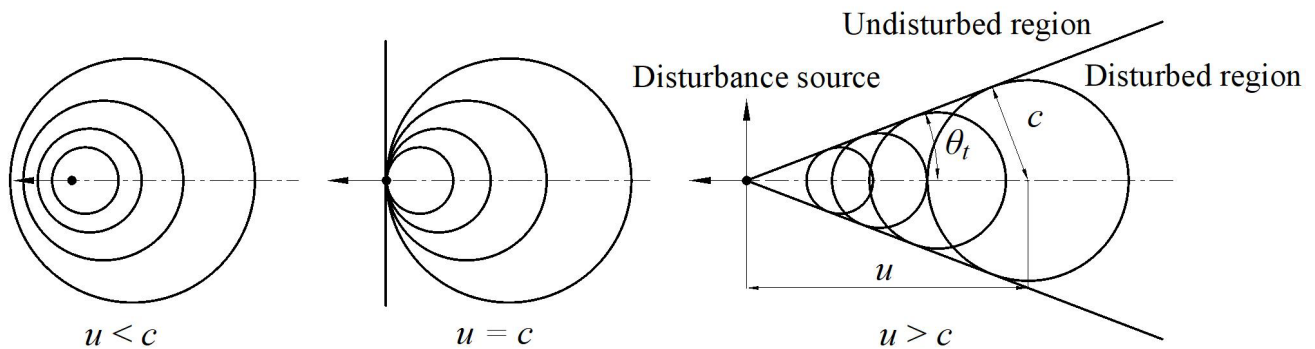
Figure 1 Propagation characteristics of disturbance in fluids
