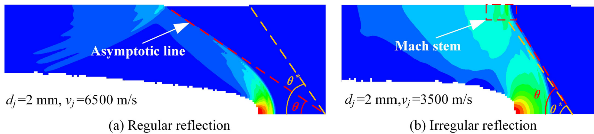
Figure 12 Distribution of shockwave pressure with different reflection types
