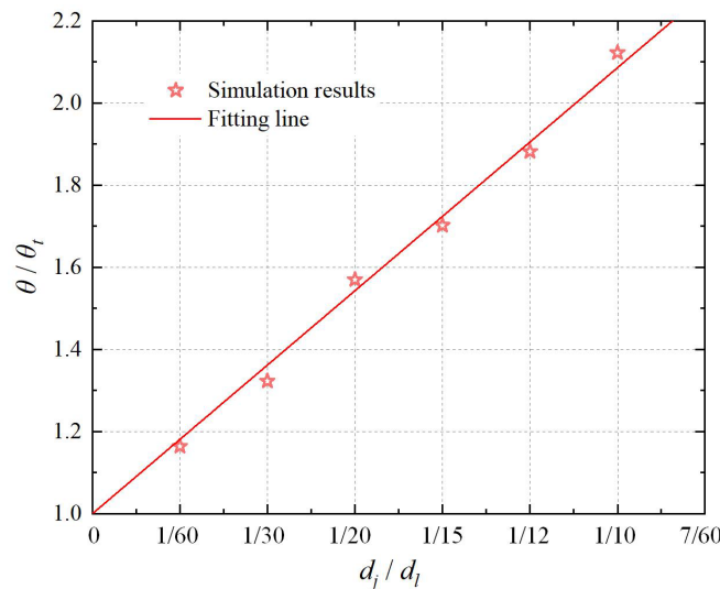
Figure 16 Trend of average value of normalized cone angle with respect to normalized diameter
