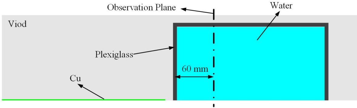
Figure 6 Schematic diagram of verification simulation model
