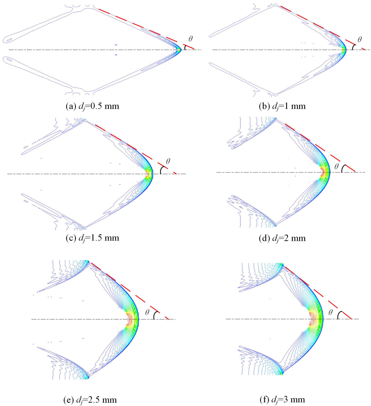
Figure 11 Shockwave in water formed by projectiles with different diameter
