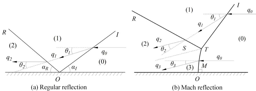
Figure 3 Diagram of shock reflection relationship (Ben-Dor 2007, Vasilev et al. 2008)
