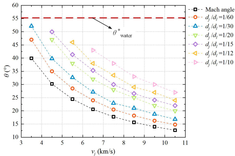
Figure 14 Variation trend of cone Angle of shockwave front with projectile velocity
