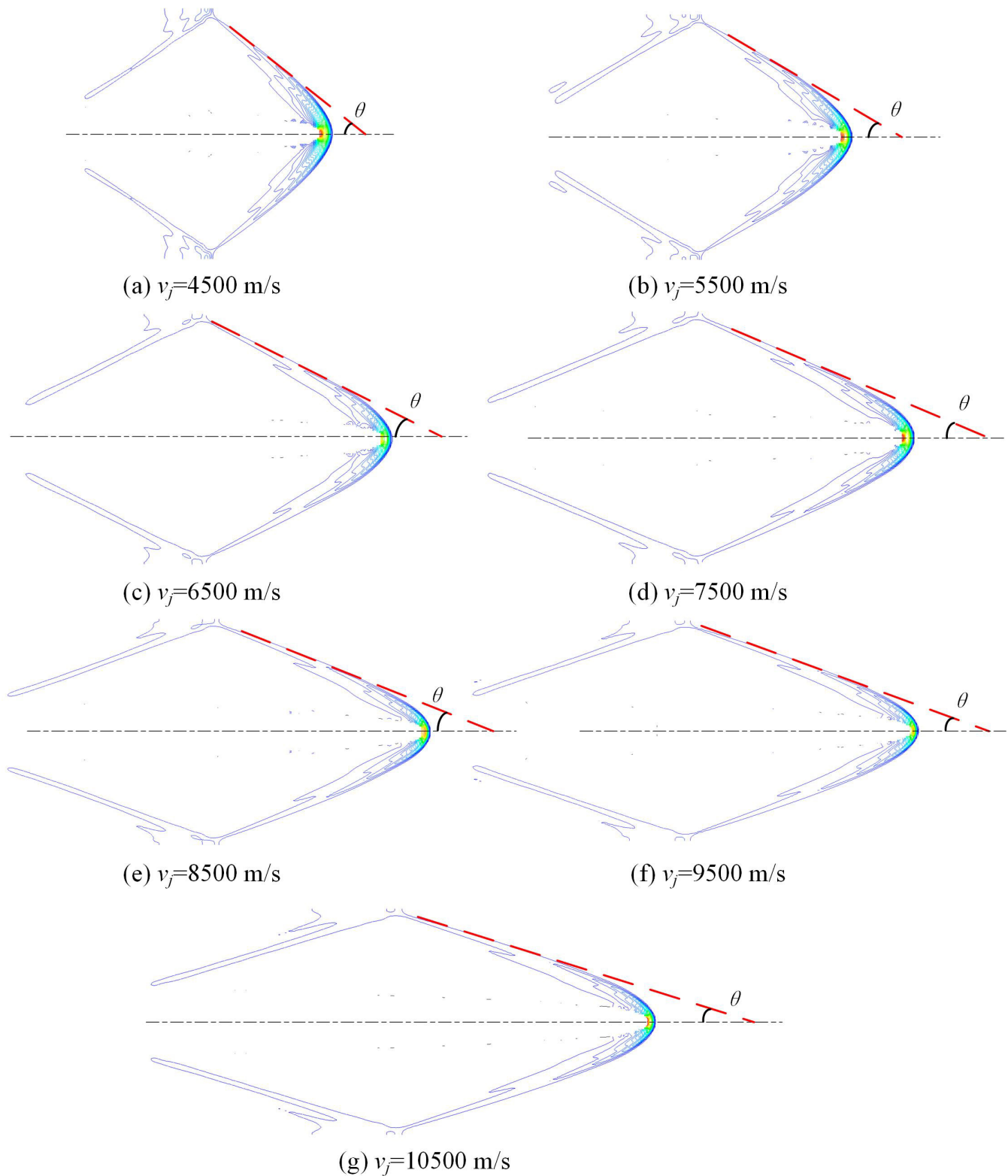
Figure 10 Shockwaves formed by projectile at different velocities
