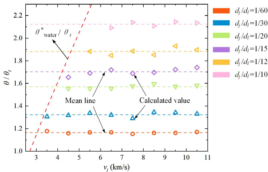
Figure 15 Variation trend of normalized cone angle versus projectile velocities
