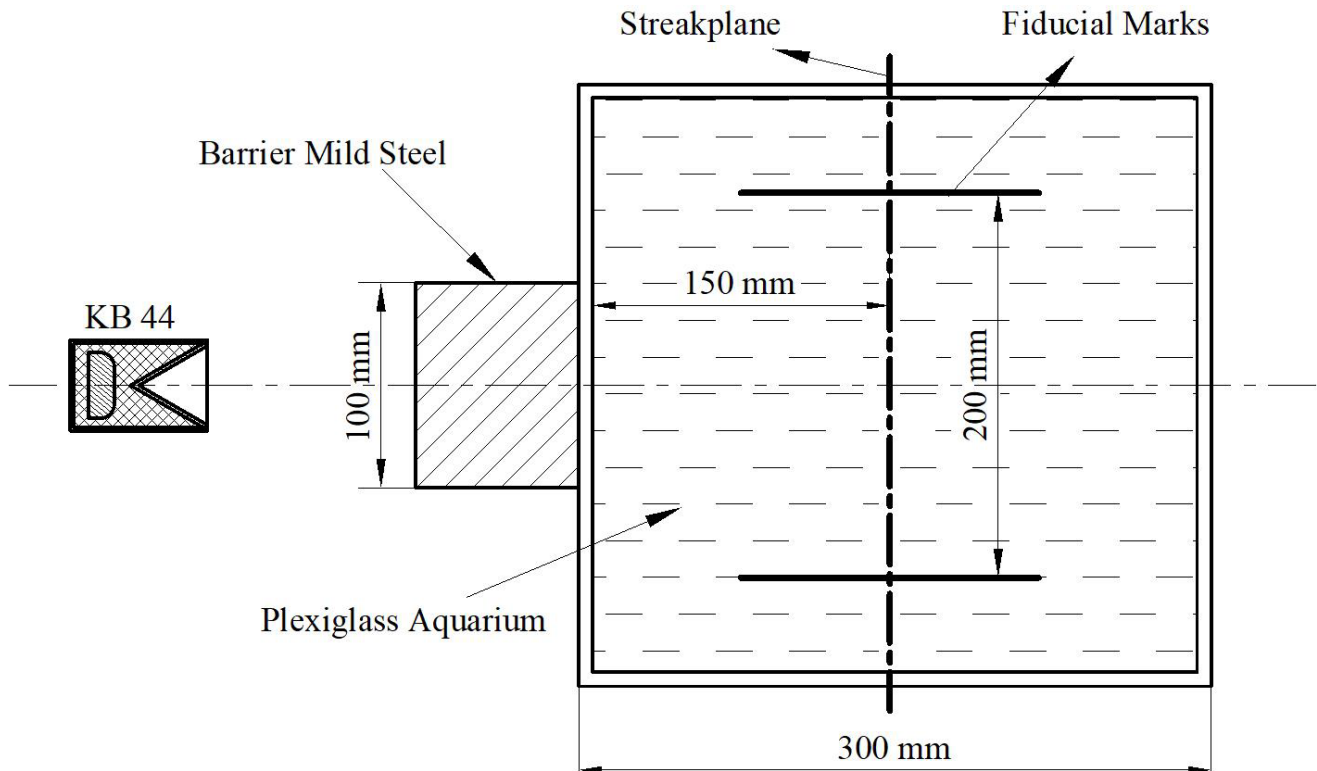
Figure 5 The layout of the experiment (Held 1995)
