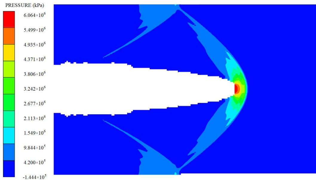
(a) Pressure distribution in water
