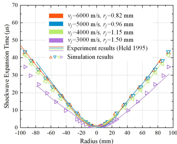
Figure 8 Comparison between simulation results and experimental results
