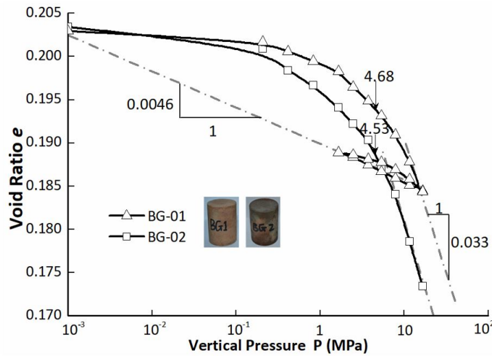
Figure 10: Test curves of e-IgP for BG-01 and BG-02.
