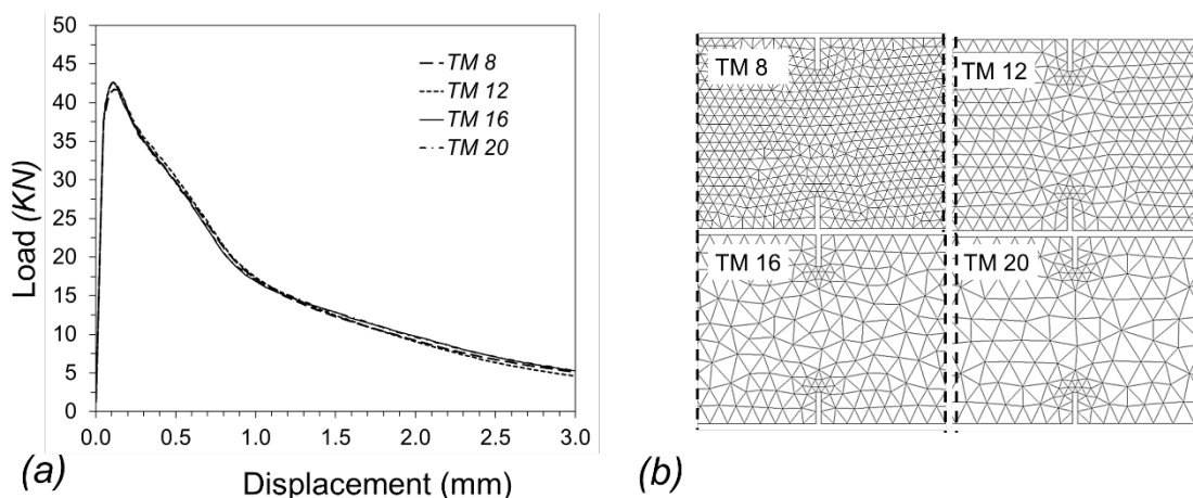
Figure 10. Influence of finite element size: (a) Curves load vs displacement for four finite element sizes (b) Four meshes used for the mesh analysis.
