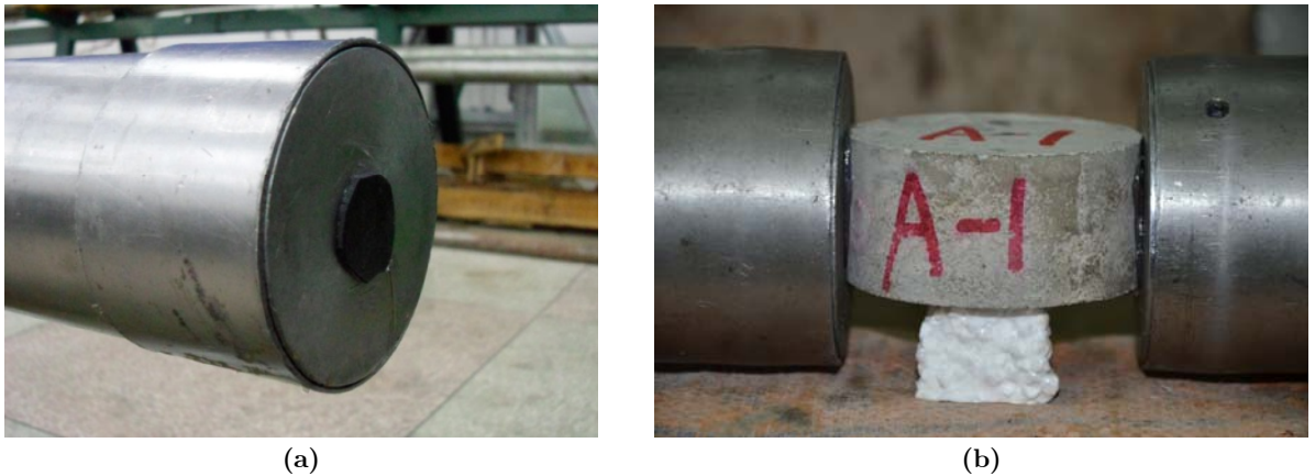
Figure 7: The position of pulse shapers and foam block under the specimen in a dynamic splitting test.
