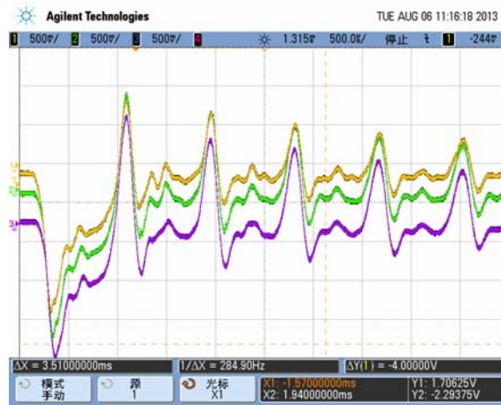
Figure 10: The original pulse signal from strain gauges on the transmitter bar in a spalling test.
