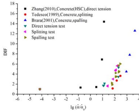
Figure 15: The influence of loading-rate on the DIF of dynamic tensile strength for concrete specimens.
