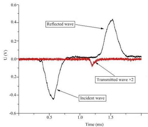
Figure 8: An original pulse signal from strain gauges in a dynamic splitting test.
