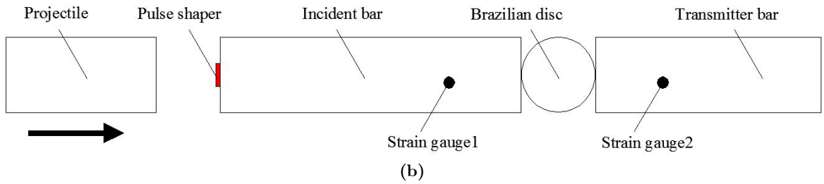
Figure 6: Illustration of the dynamic splitting test set-up.
